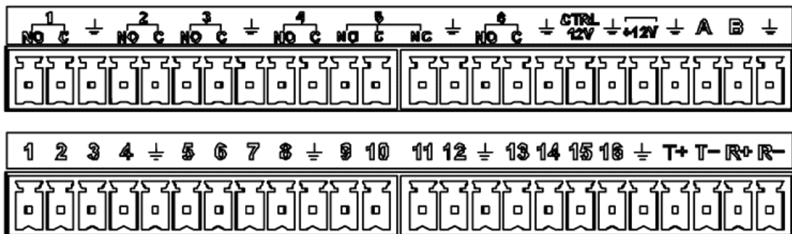
Figure 6-1 Alarm interface
