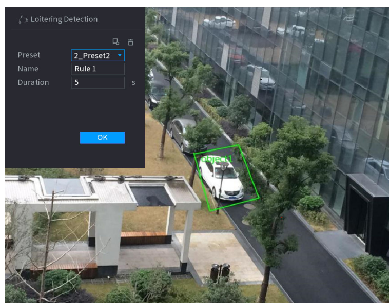
Figure 4-2 Loitering detection
