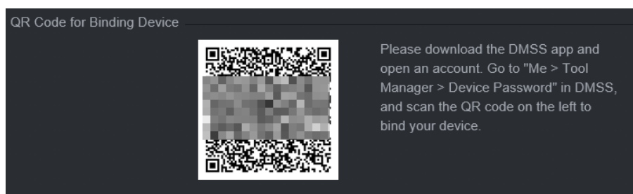
Figure 5-4 Bind device
