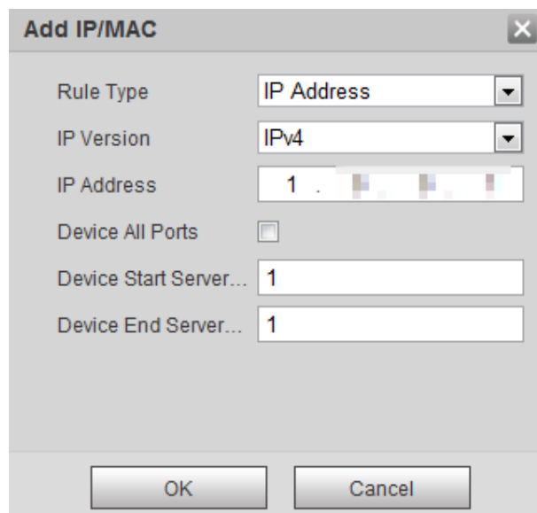
Figure 3-3 Add IP/MAC
