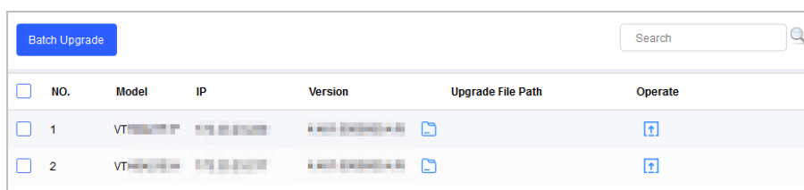
Figure 7-2 Device upgrade
