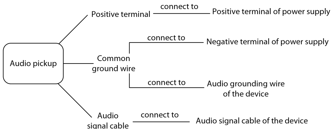
Figure 2-1 Wiring of the audio pickup
