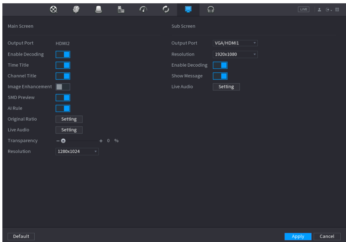
Figure 6-4 Display
