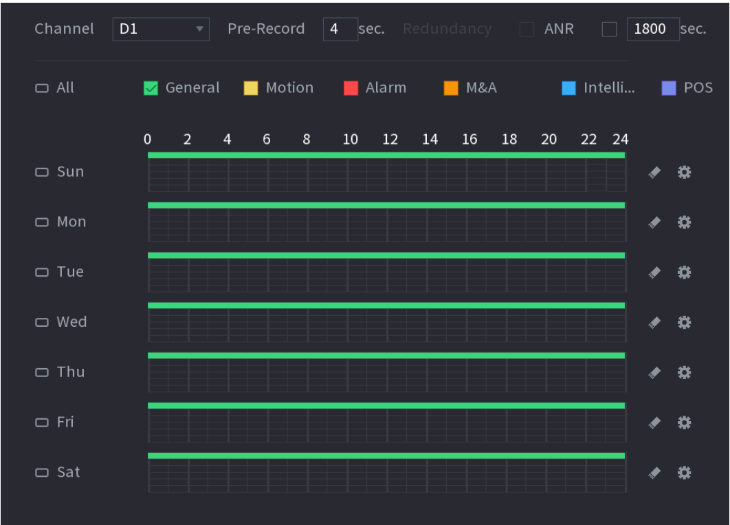
Figure 1-2 Video schedule
