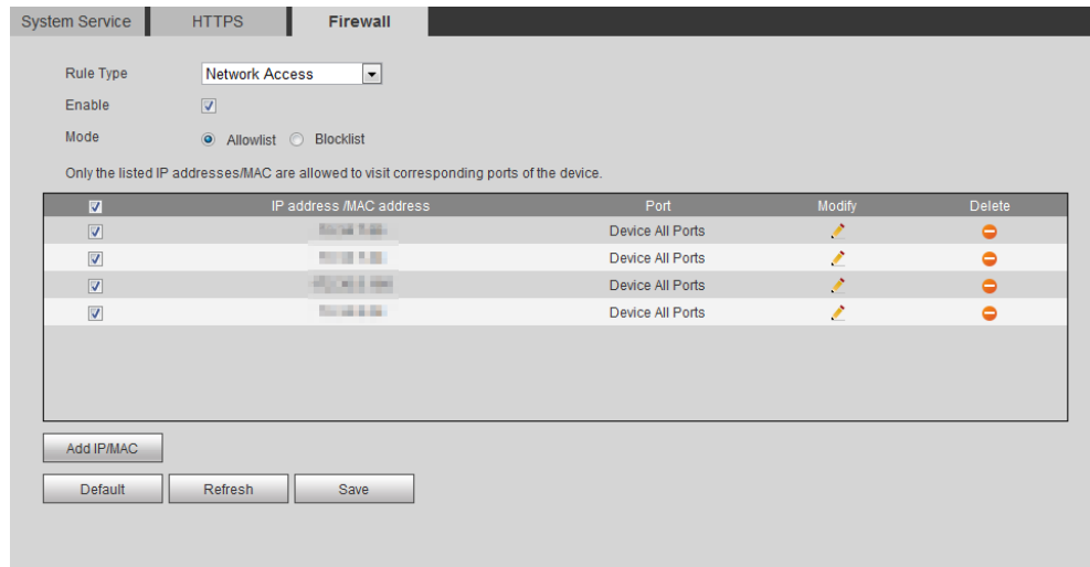
Figure 3-2 Network Access
