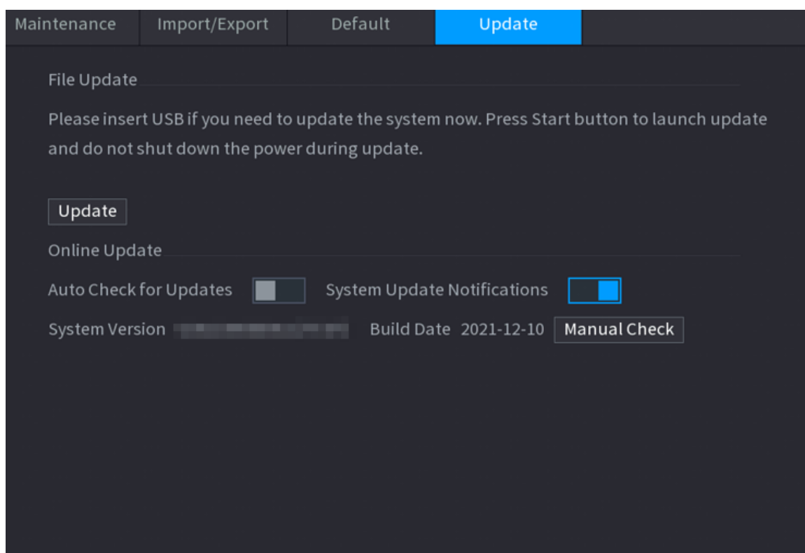
Figure 7-1 System update
