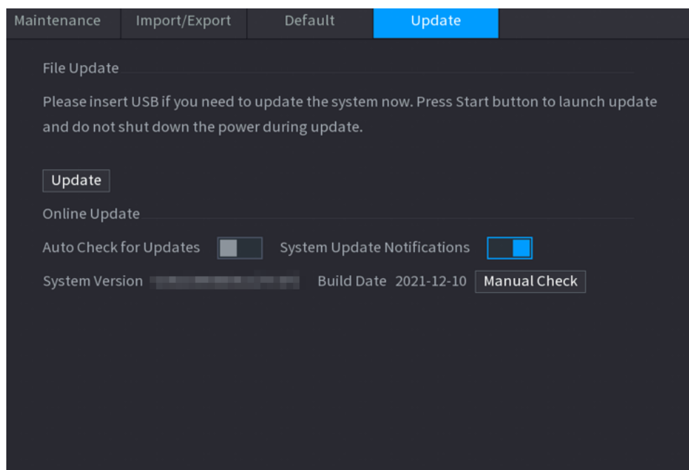
Figure 1-5 Update
