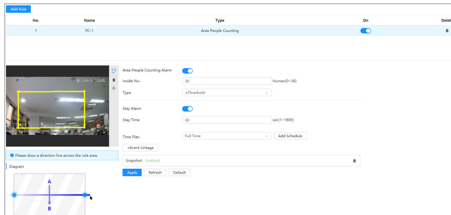
Figure 9-4 Add an area people counting rule
