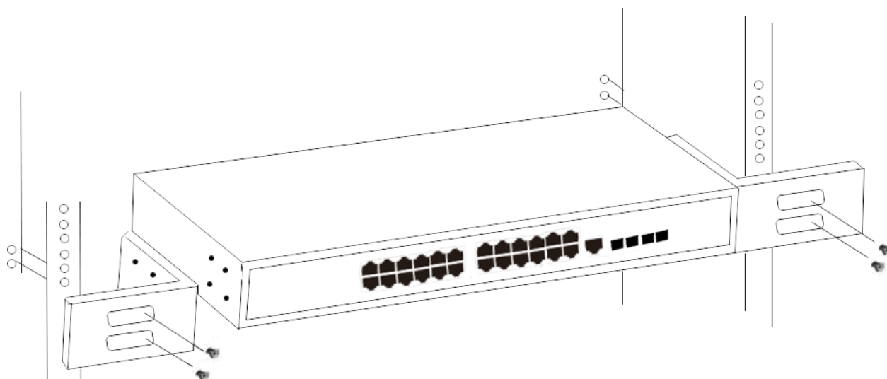
Figure 4 - Rack Installation
